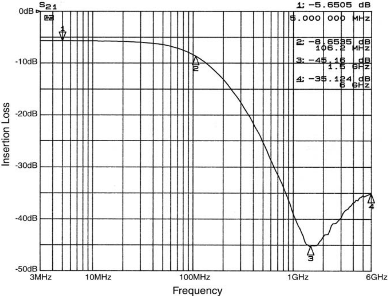
Typical Insertion Loss vs. Frequency curve:
